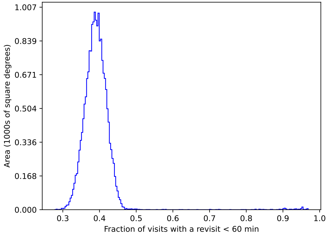
weather_cloudso12v3.4_10yrs gri WFD: Fraction of visits with a revisit < 60 min
