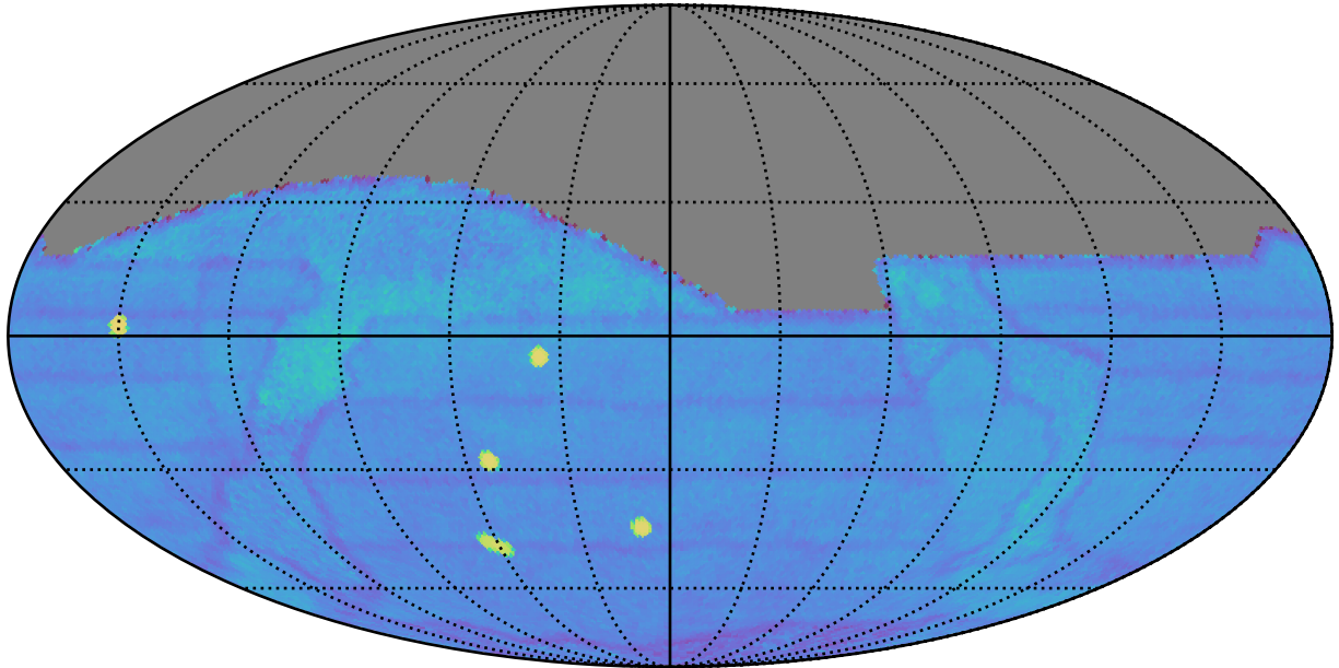
weather_cloudso12v3.4_10yrs gri All sky: Fraction of visits with a revisit < 60 min
