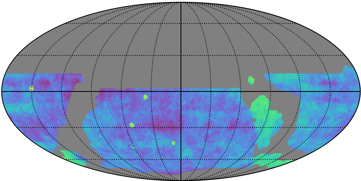
weather_cloudso12v3.4_10yrs gri WFD: Fraction of visits in pairs (20-90 min)
