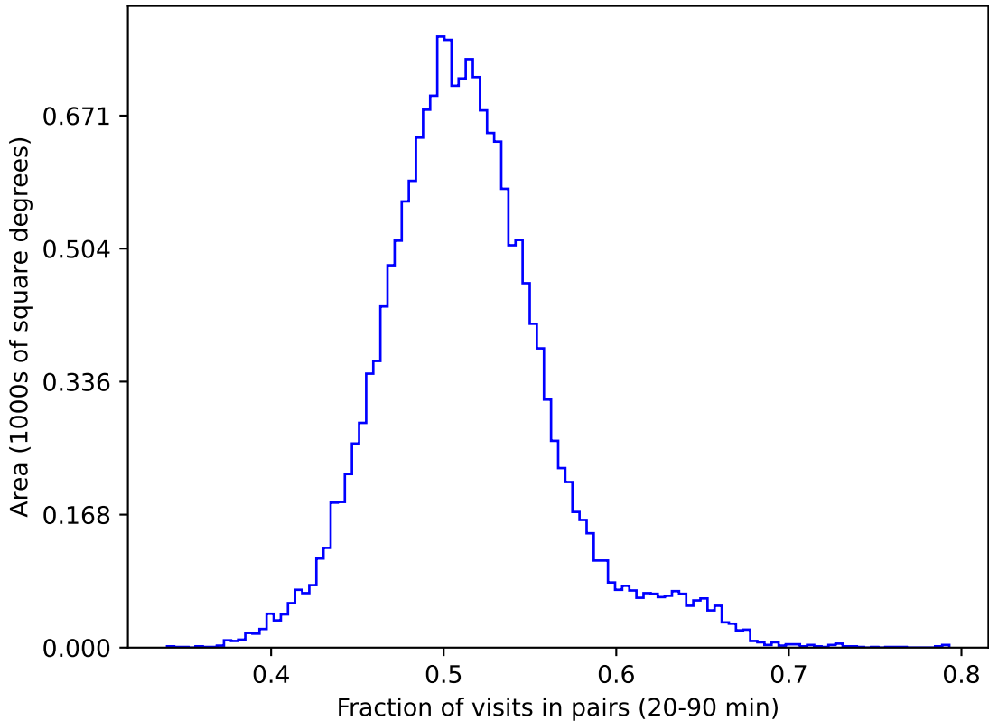
weather_cloudso12v3.4_10yrs gri WFD: Fraction of visits in pairs (20-90 min)
