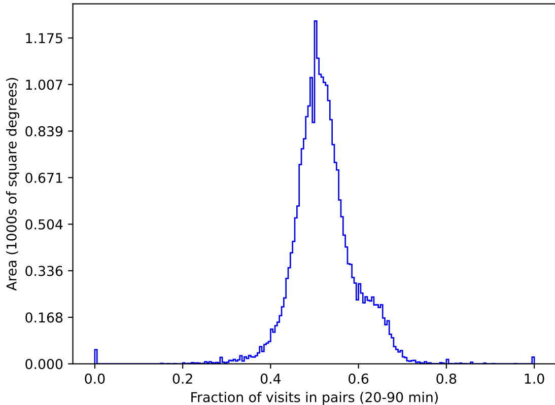
weather_cloudso12v3.4_10yrs gri All sky: Fraction of visits in pairs (20-90 min)
