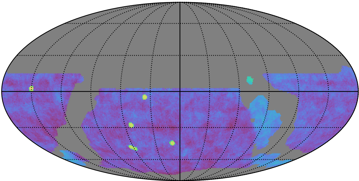
weather_cloudso12v3.4_10yrs gri WFD: Fraction of visits in pairs (10-60 min)
