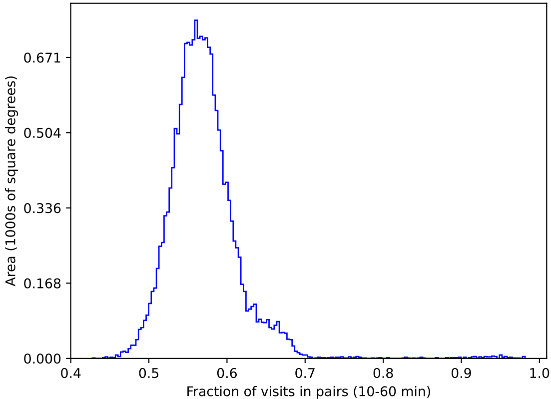
weather_cloudso12v3.4_10yrs gri WFD: Fraction of visits in pairs (10-60 min)
