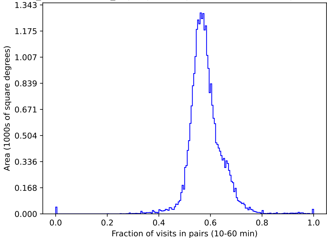
weather_cloudso12v3.4_10yrs gri All sky: Fraction of visits in pairs (10-60 min)
