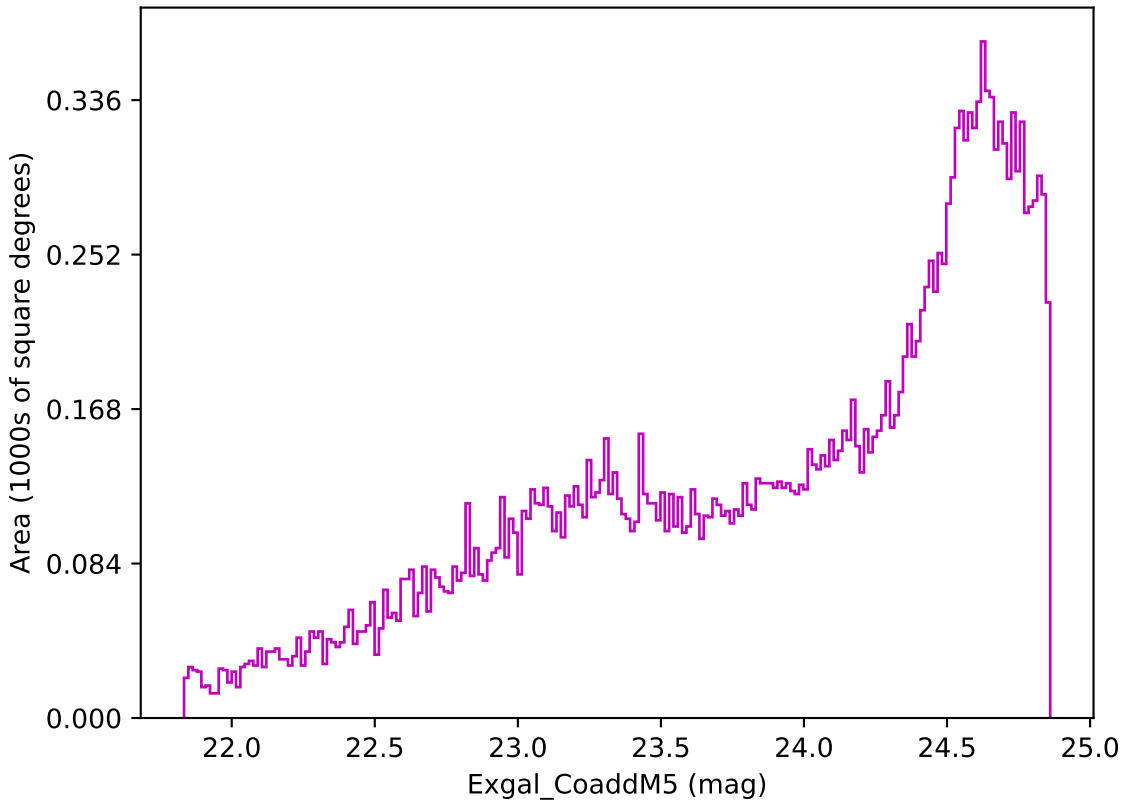
weather_cloudso12v3.4_10yrs Yr 3-4 z band: Exgal_CoaddM5
