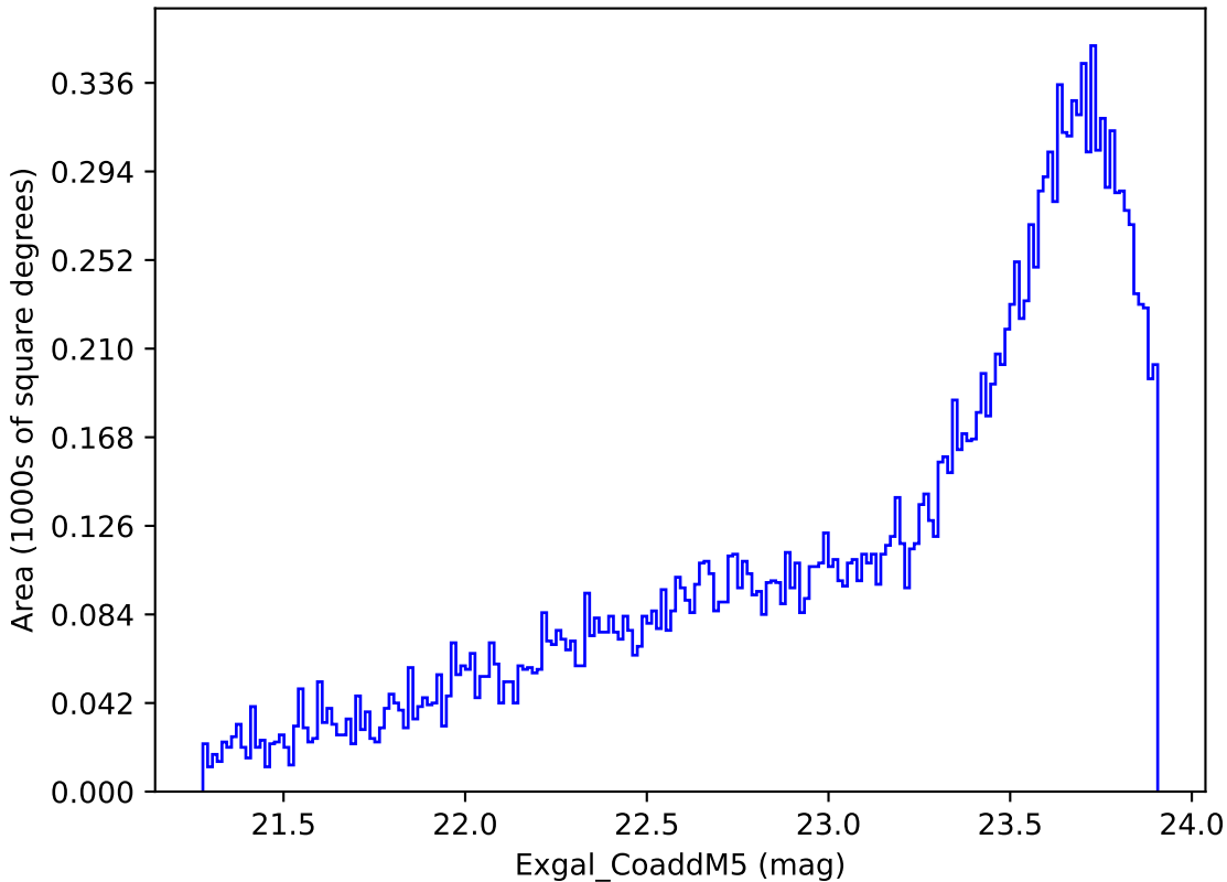
weather_cloudso12v3.4_10yrs Yr 3-4 y band: Exgal_CoaddM5
