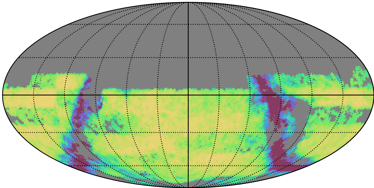
weather_cloudso12v3.4_10yrs Yr 3-4 u band: Exgal_CoaddM5
