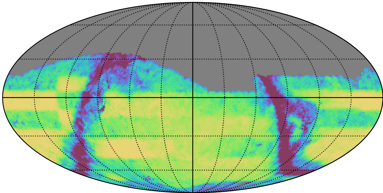
weather_cloudso12v3.4_10yrs Yr 3-4 r band: Exgal_CoaddM5
