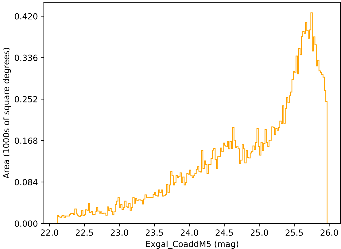
weather_cloudso12v3.4_10yrs Yr 3-4 r band: Exgal_CoaddM5
