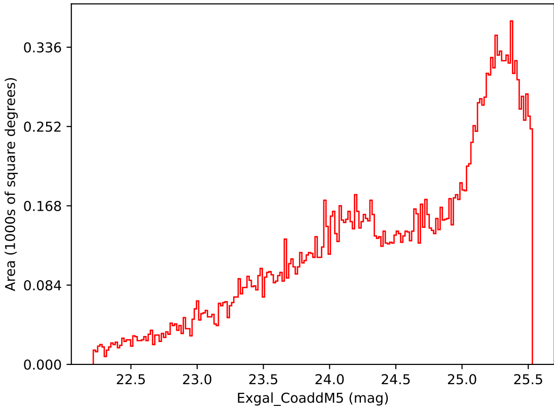
weather_cloudso12v3.4_10yrs Yr 3-4 i band: Exgal_CoaddM5
