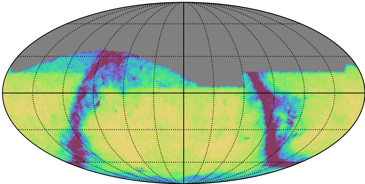
weather_cloudso12v3.4_10yrs Yr 1 r band: Exgal_CoaddM5
