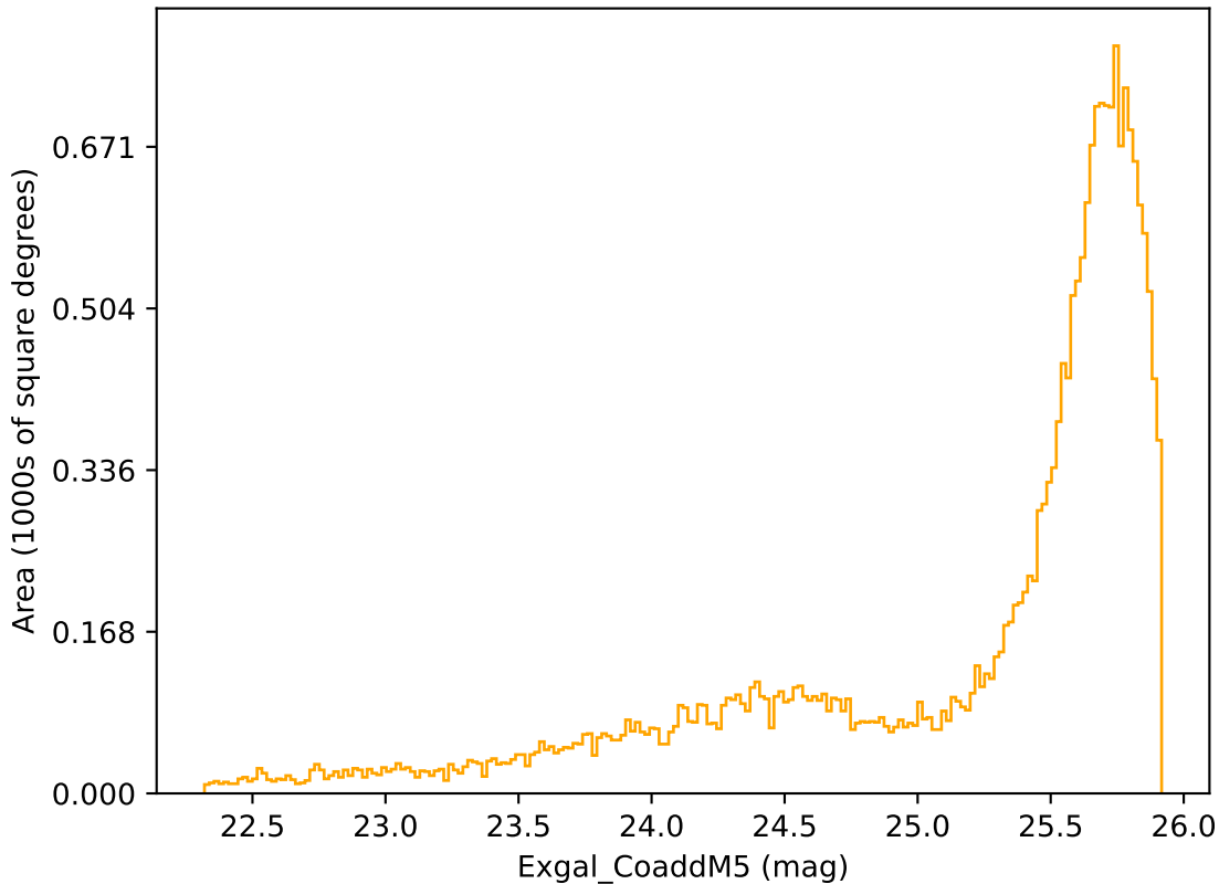
weather_cloudso12v3.4_10yrs Yr 1 r band: Exgal_CoaddM5
