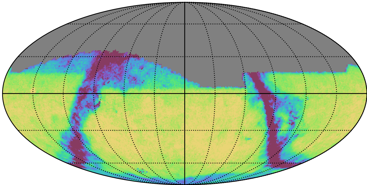
weather_cloudso12v3.4_10yrs Yr 1 i band: Exgal_CoaddM5
