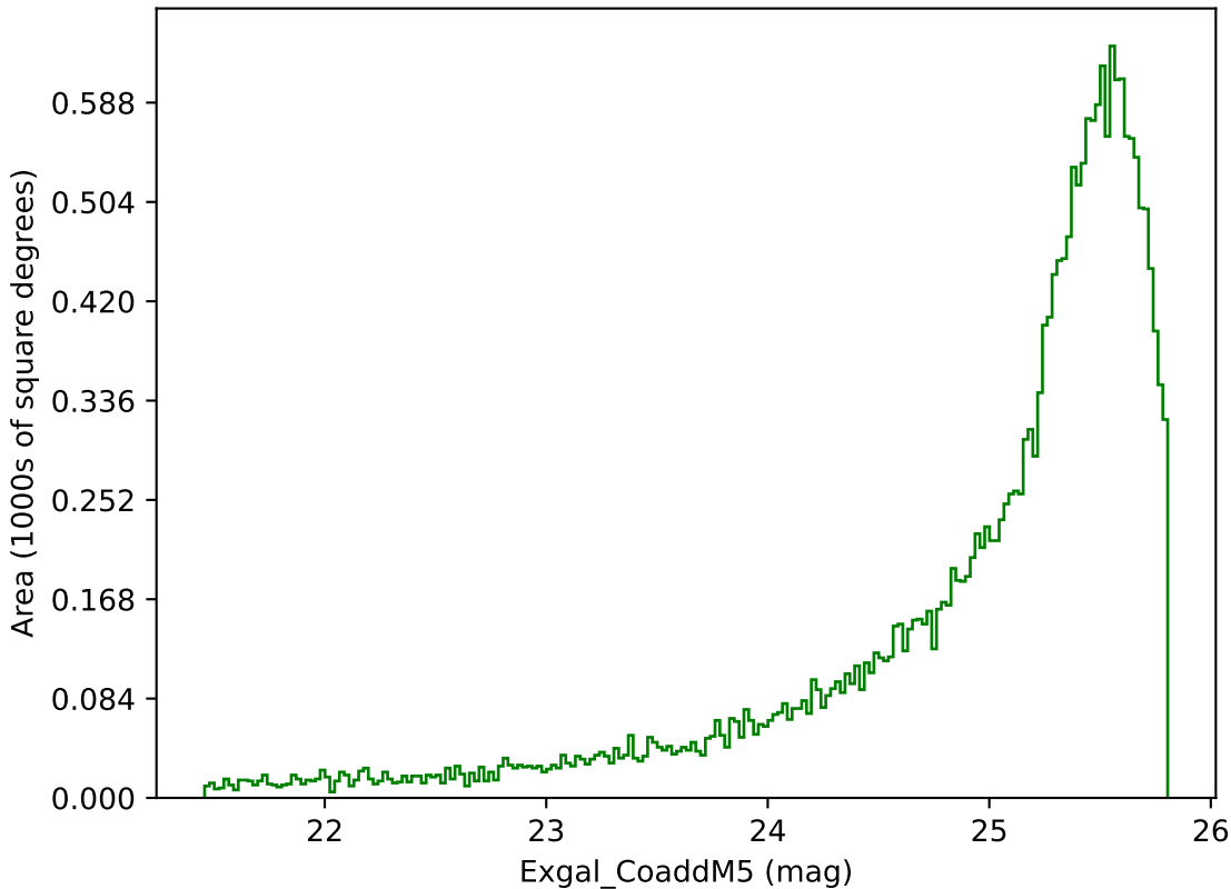
weather_cloudso12v3.4_10yrs Yr 1 g band: Exgal_CoaddM5
