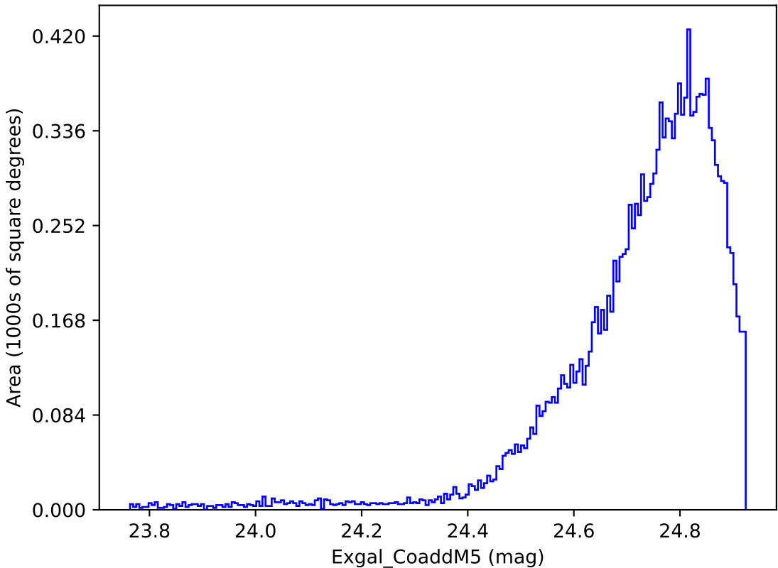
weather_cloudso12v3.4_10yrs WFD y band: Exgal_CoaddM5
