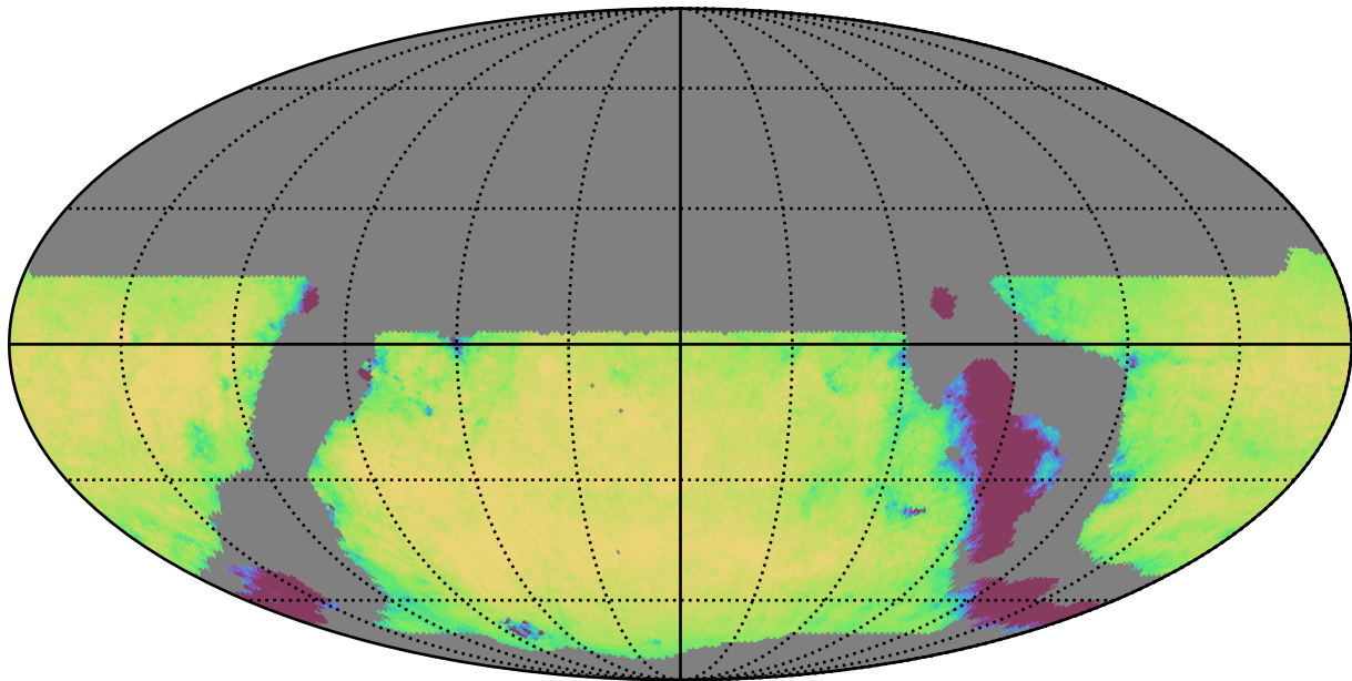
weather_cloudso12v3.4_10yrs WFD u band: Exgal_CoaddM5
