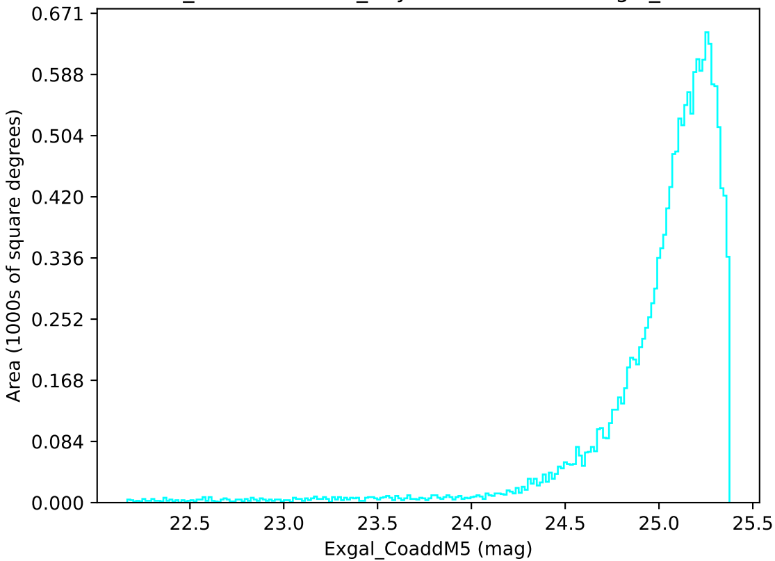
weather_cloudso12v3.4_10yrs WFD u band: Exgal_CoaddM5
