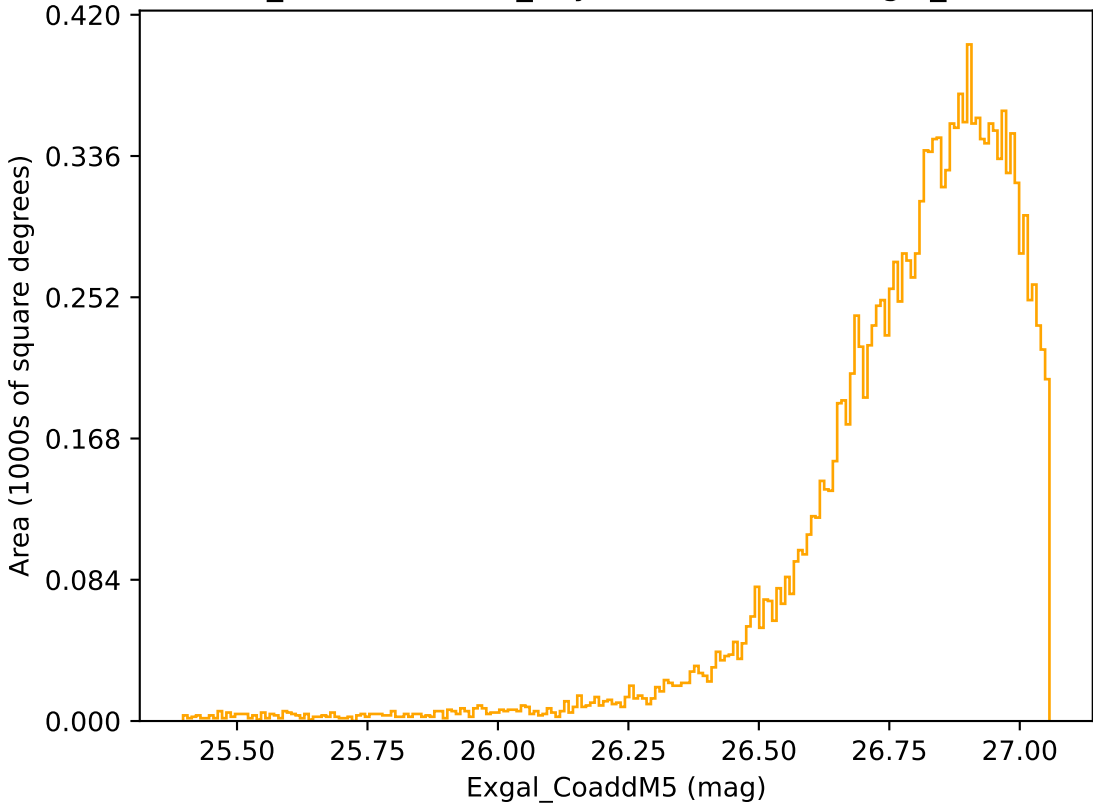
weather_cloudso12v3.4_10yrs WFD r band: Exgal_CoaddM5
