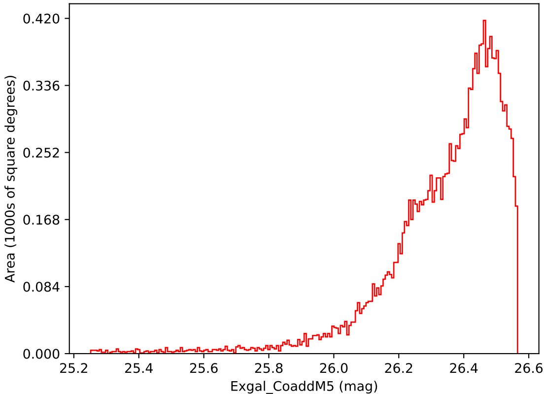
weather_cloudso12v3.4_10yrs WFD i band: Exgal_CoaddM5
