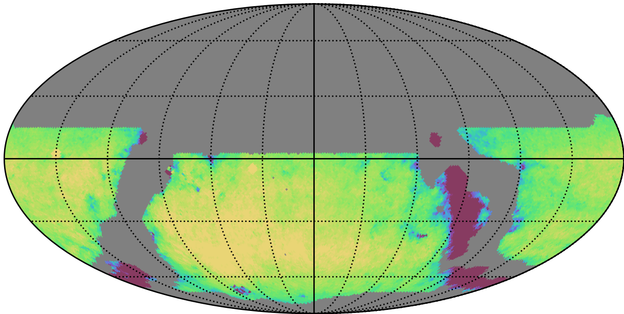
weather_cloudso12v3.4_10yrs WFD g band: Exgal_CoaddM5
