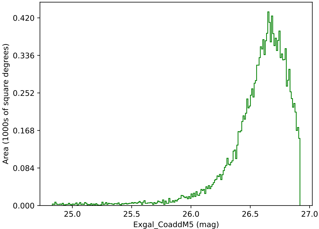
weather_cloudso12v3.4_10yrs WFD g band: Exgal_CoaddM5
