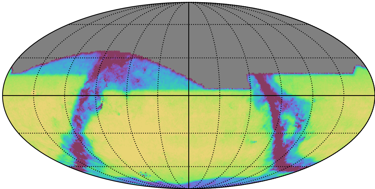
weather_cloudso12v3.4_10yrs All sky z band: Exgal_CoaddM5
