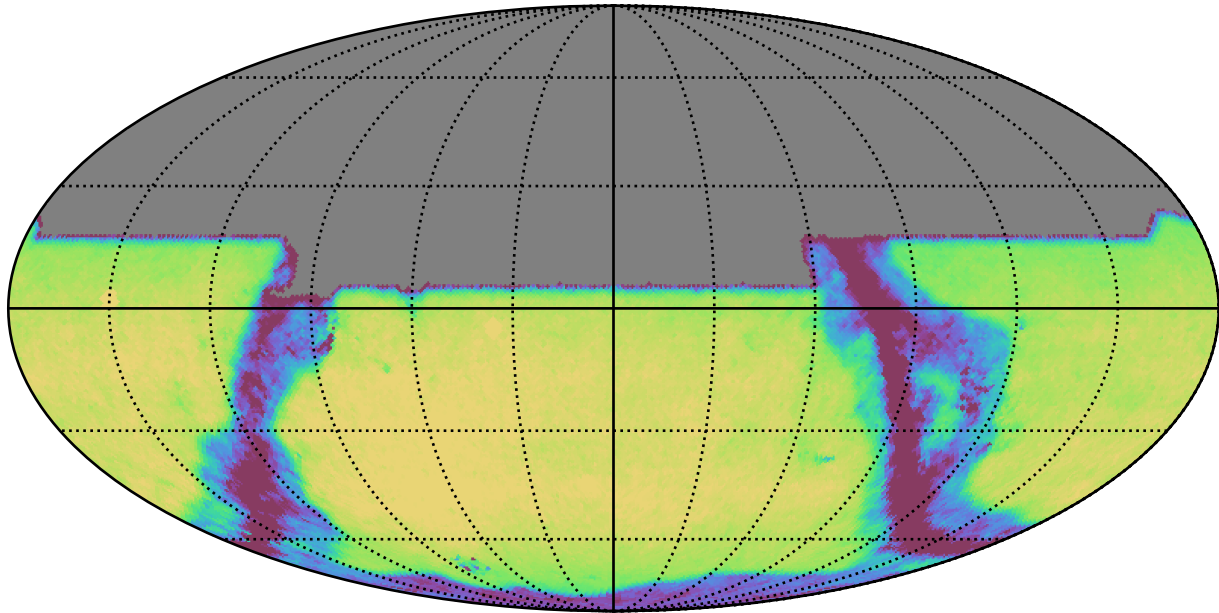
weather_cloudso12v3.4_10yrs All sky y band: Exgal_CoaddM5
