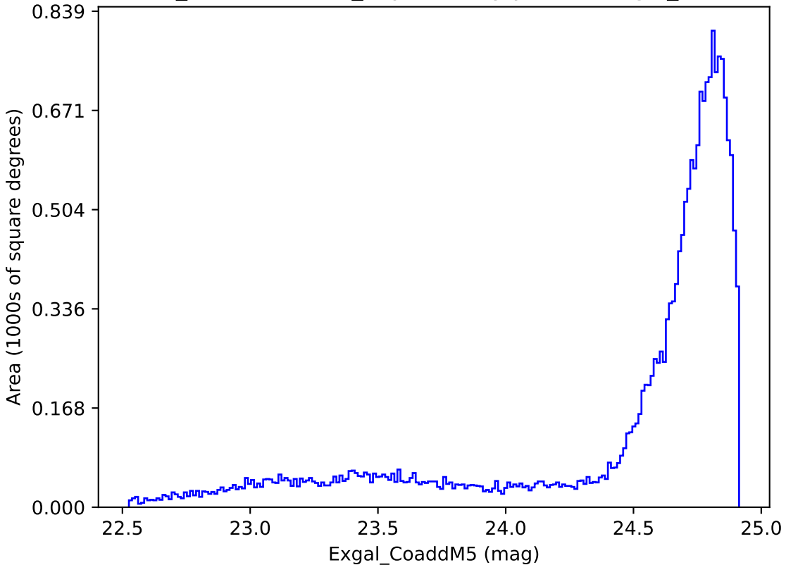
weather_cloudso12v3.4_10yrs All sky y band: Exgal_CoaddM5
