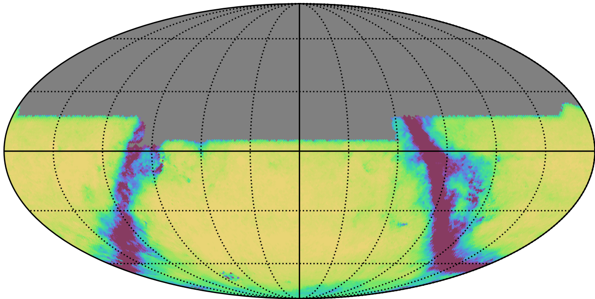
weather_cloudso12v3.4_10yrs All sky u band: Exgal_CoaddM5
