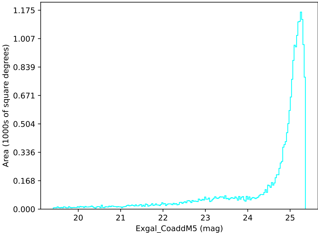
weather_cloudso12v3.4_10yrs All sky u band: Exgal_CoaddM5
