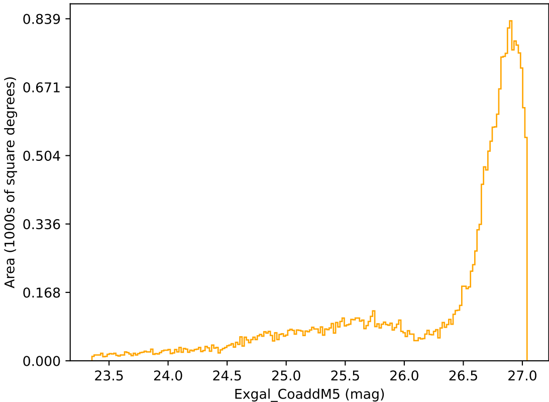
weather_cloudso12v3.4_10yrs All sky r band: Exgal_CoaddM5
