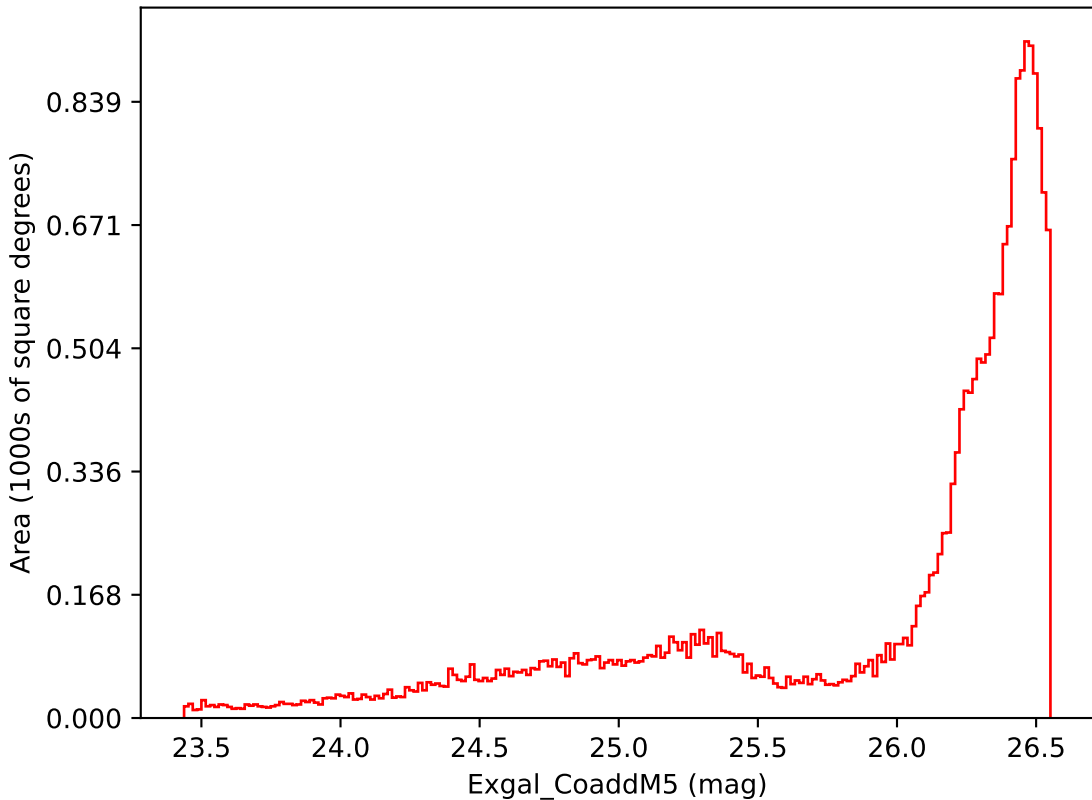
weather_cloudso12v3.4_10yrs All sky i band: Exgal_CoaddM5
