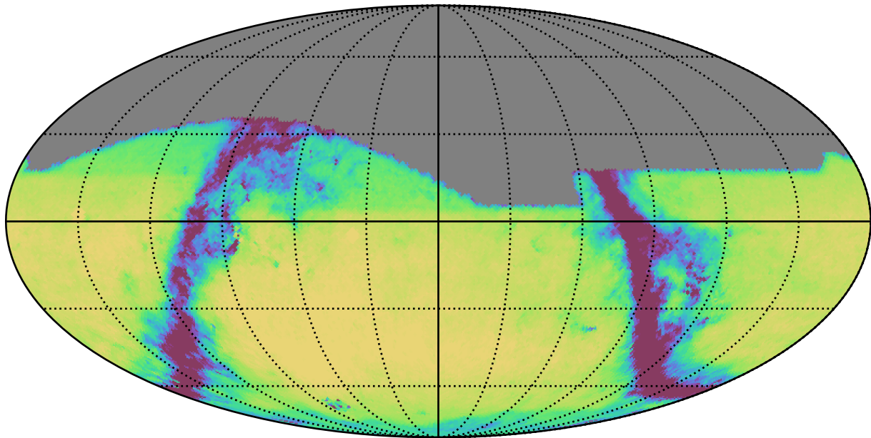
weather_cloudso12v3.4_10yrs All sky g band: Exgal_CoaddM5
