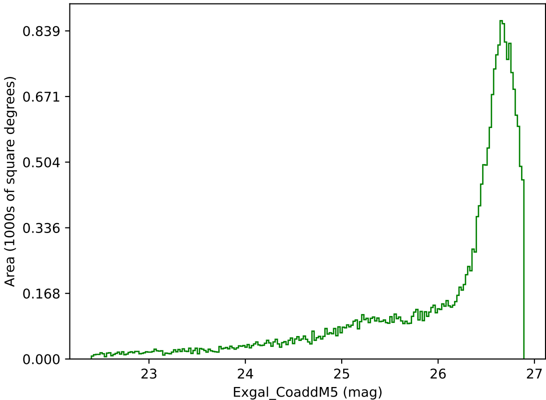
weather_cloudso12v3.4_10yrs All sky g band: Exgal_CoaddM5
