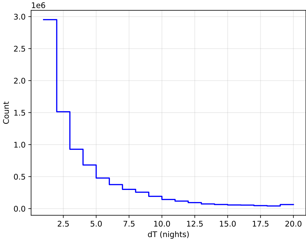
weather_cloudso12v3.4_10yrs WFD all bands: DeltaNight Histogram
