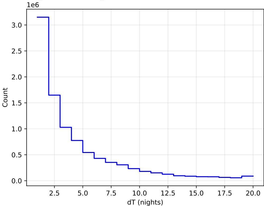
weather_cloudso12v3.4_10yrs All sky all bands: DeltaNight Histogram
