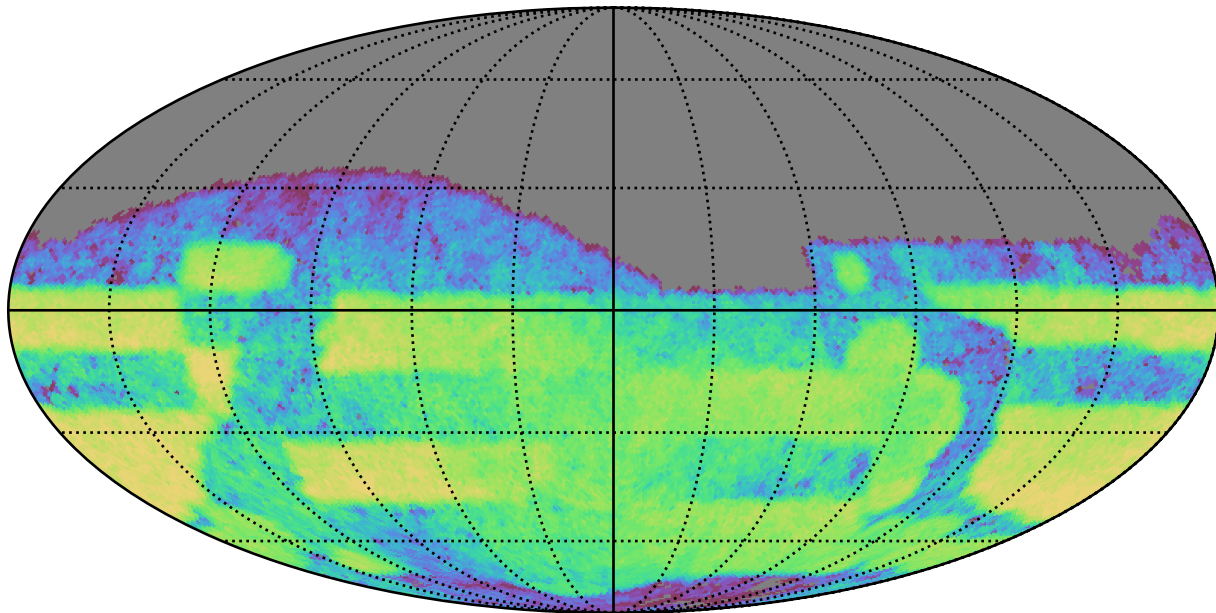
weather_cloudso12v3.4_10yrs Yr 3-4 r band: CoaddM5
