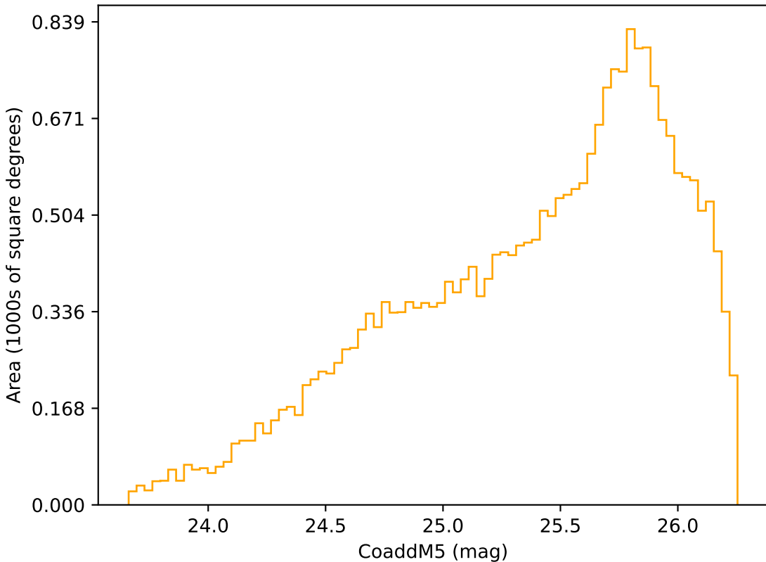
weather_cloudso12v3.4_10yrs Yr 3-4 r band: CoaddM5
