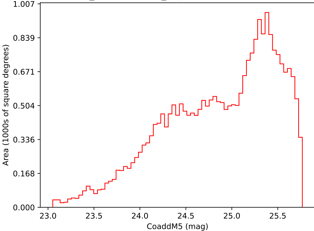
weather_cloudso12v3.4_10yrs Yr 3-4 i band: CoaddM5
