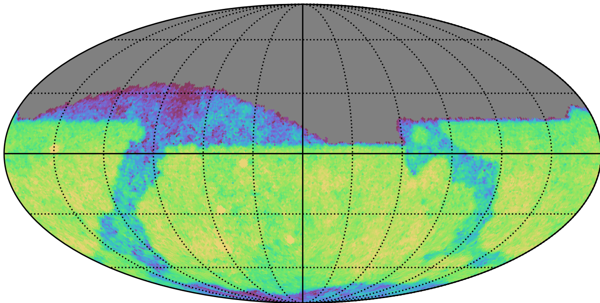
weather_cloudso12v3.4_10yrs Yr 1 z band: CoaddM5
