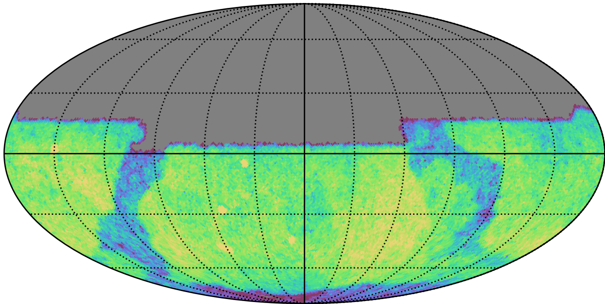
weather_cloudso12v3.4_10yrs Yr 1 y band: CoaddM5
