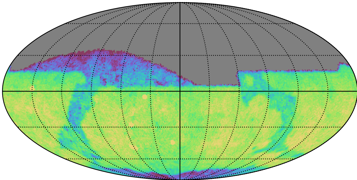
weather_cloudso12v3.4_10yrs Yr 1 r band: CoaddM5
