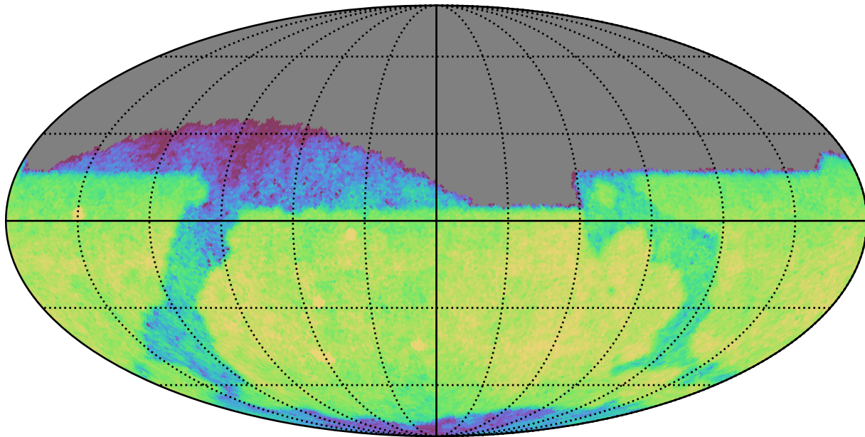
weather_cloudso12v3.4_10yrs Yr 1 i band: CoaddM5
