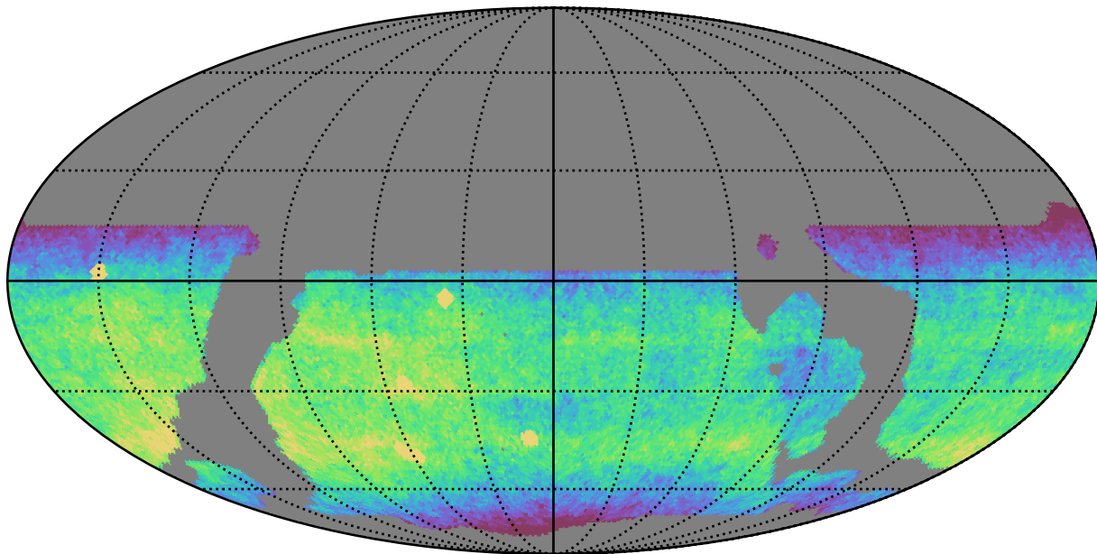
weather_cloudso12v3.4_10yrs WFD z band: CoaddM5
