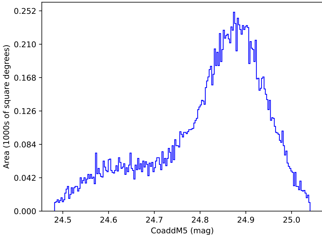
weather_cloudso12v3.4_10yrs WFD y band: CoaddM5
