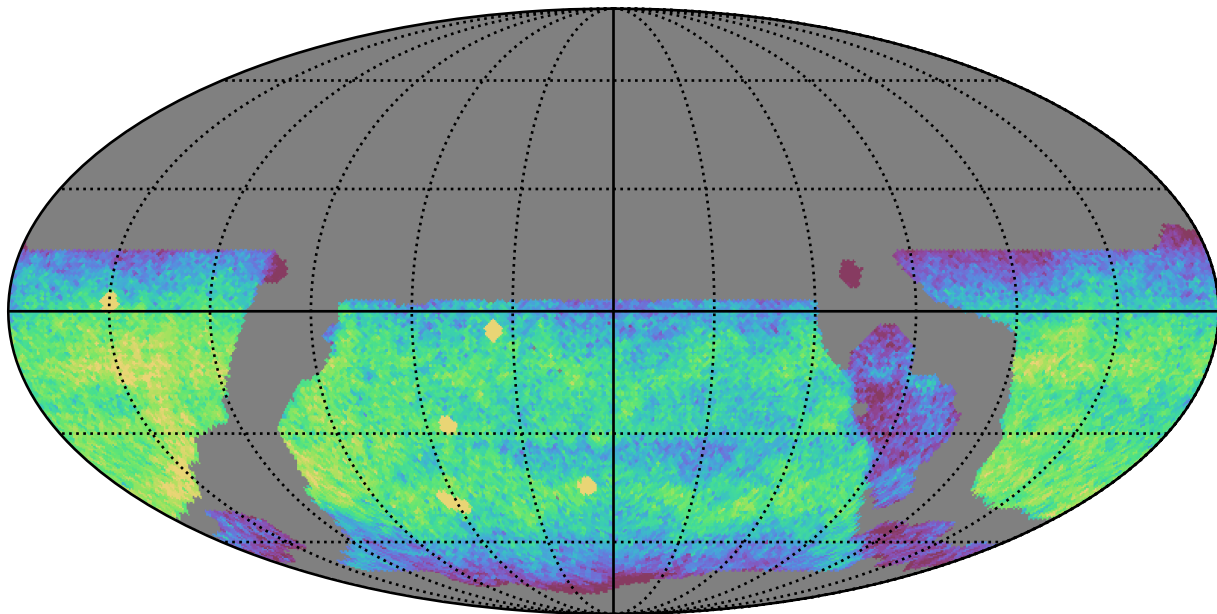
weather_cloudso12v3.4_10yrs WFD u band: CoaddM5
