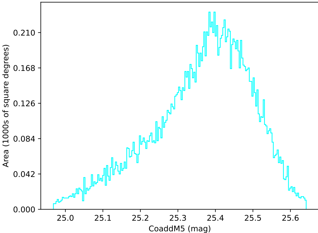
weather_cloudso12v3.4_10yrs WFD u band: CoaddM5
