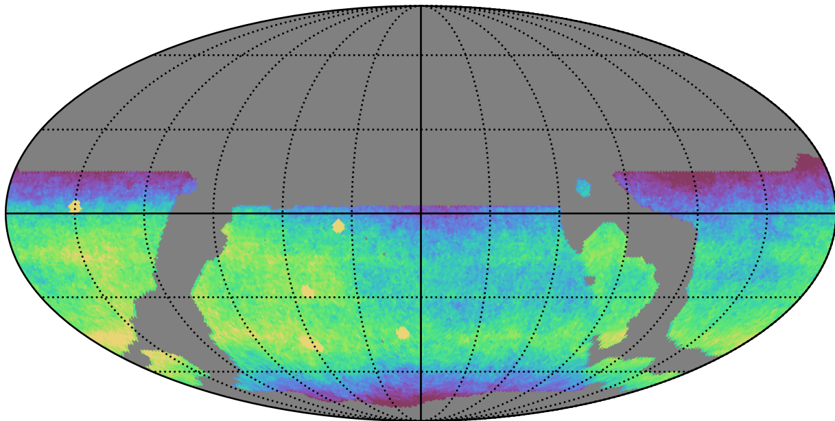
weather_cloudso12v3.4_10yrs WFD r band: CoaddM5
