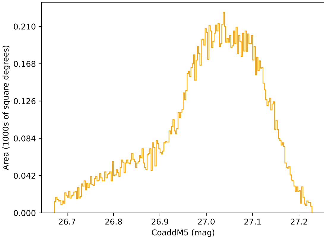
weather_cloudso12v3.4_10yrs WFD r band: CoaddM5
