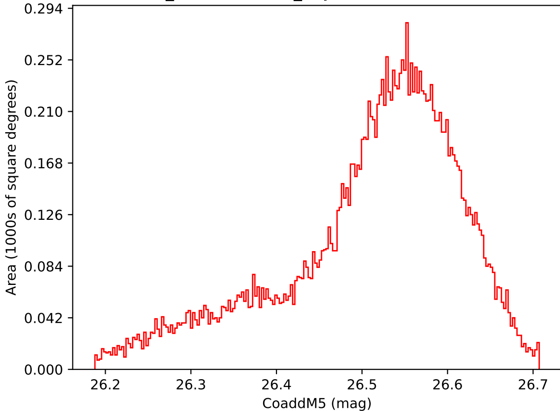
weather_cloudso12v3.4_10yrs WFD i band: CoaddM5
